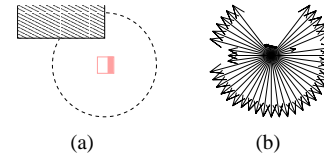
Fig. 3. (a) Detection of convex landmarks from a single position. (b) Using a ring of 48 sonar sensors.
